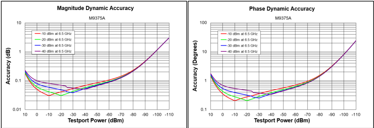
Dynamic accuracy, 6.5 GHz ( magnitude and phase )
